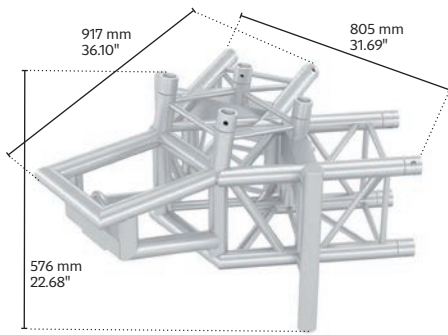
MRT1-01B|BaseCorner
