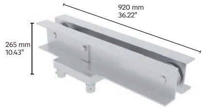
MRT1-02B|HeadSection
