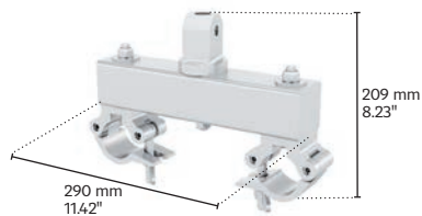
MRT1-04|StabilizerHorizontalR
