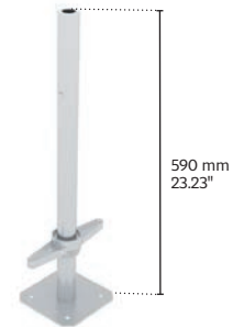
ScrewjackTR38x1-590
