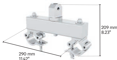
MRT1-04|StabilizerHorizontalL
