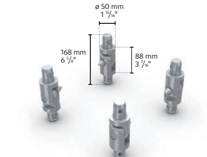
MRT1-07B|Hinges|4pcs
