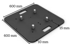
CM/CF-BP-STEEL-600x600
