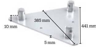
3CF30-WPC
