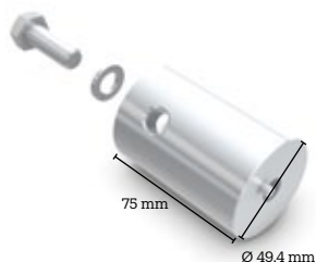
CON338
