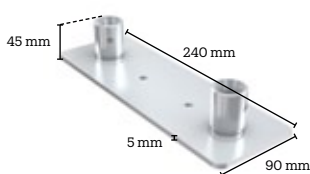
2CM22-WP
