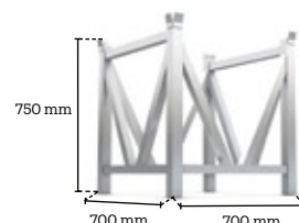
TRA-CAG-BP-600x600x10
