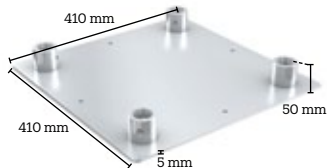
4CF40H-WP
