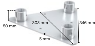
3CF30-WP
