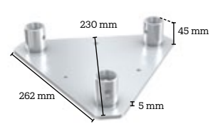
3CM22-WP
