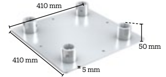
4CF30-WP
